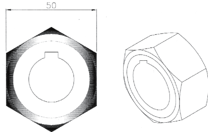
Hexagon Adapter
