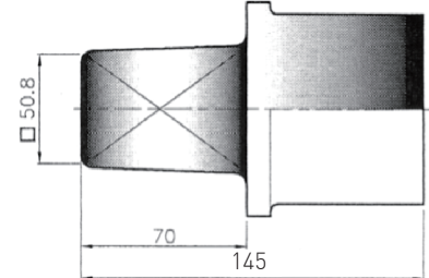
2" Square Nut
