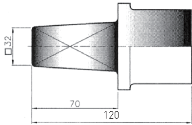
32 Square Nut
